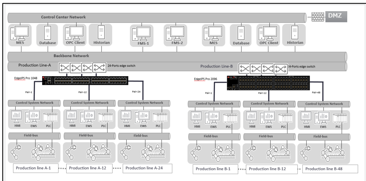
Figure 1. TXOne Security Solutions for an OT Network
