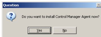
FIGURE 2-16. Question dialog
