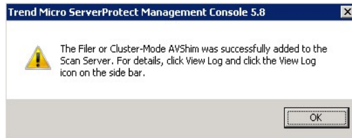
FIGURE 3-38. Confirmation screen
