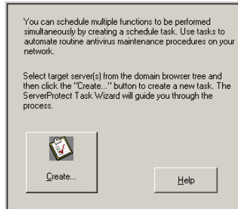
FIGURE 3-32. Configuration Area
