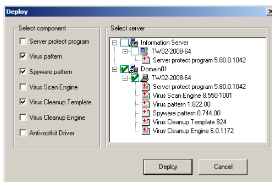
FIGURE 3-48. Deploy dialog
