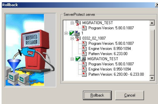
FIGURE 3-51. Rollback dialog
