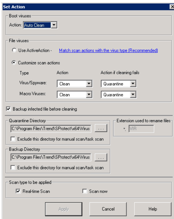
FIGURE 3-28. Set Action dialog for Normal Server
