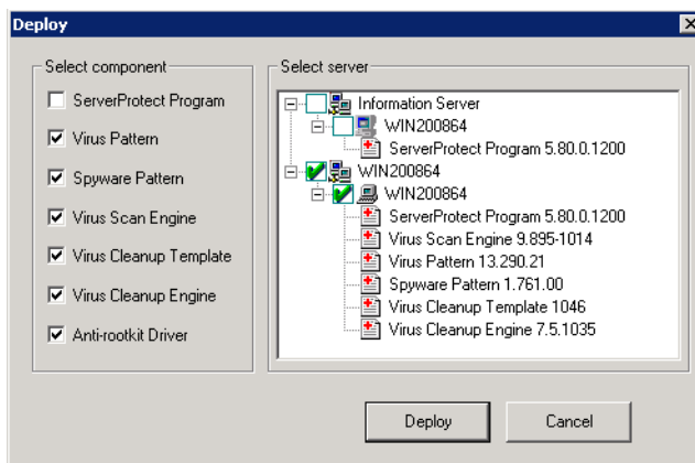
FIGURE 3-11. Deploy dialog
