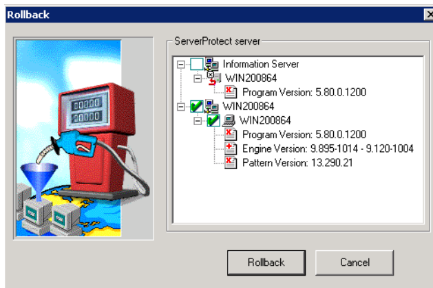
FIGURE 3-14. Rollback dialog
