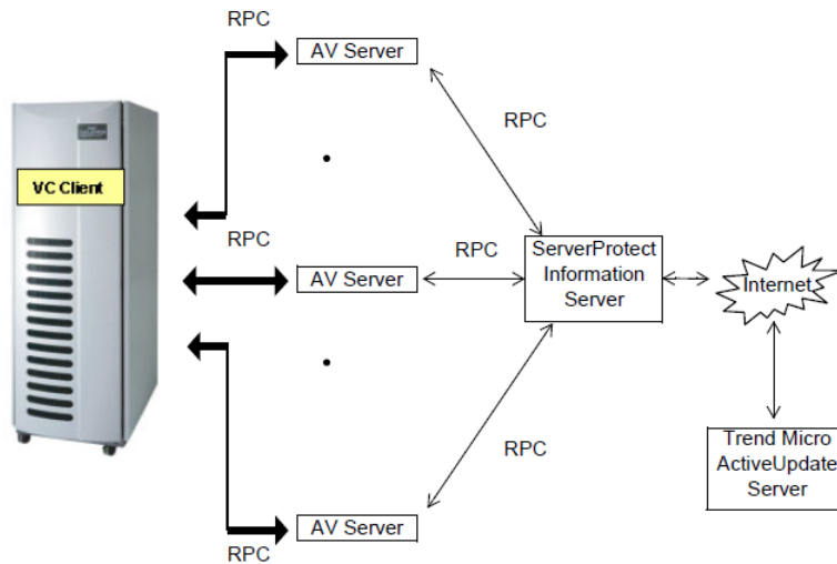
FIGURE 1-3. ServerProtect for EMC Celerra Organizational Flow
