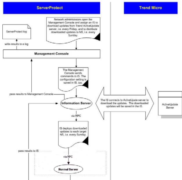
FIGURE 3-6. How Updates Work
