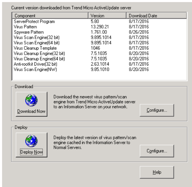
FIGURE 3-7. Trend Micro ServerProtect Update Main Screen
