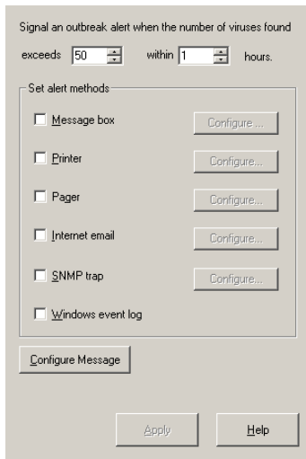
FIGURE 3-26. ServerProtect Outbreak Alert Events Configuration Window
