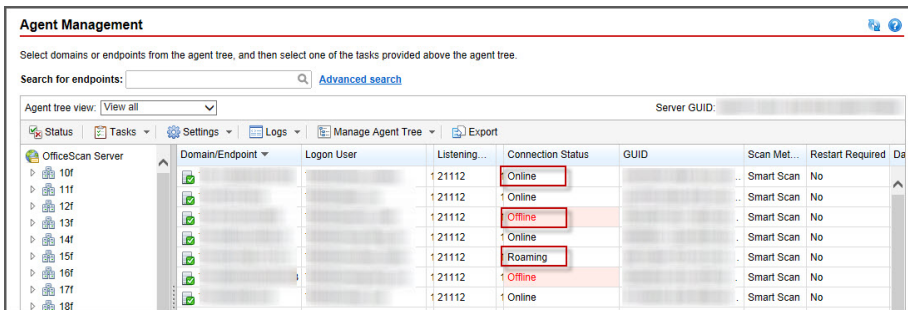
FIGURE 15-2. Agent tree displaying agent connection status with OfficeScan server
