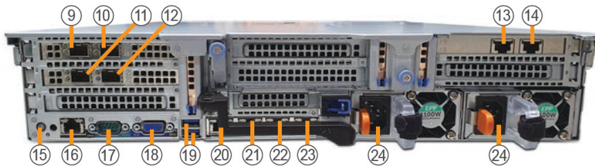
FIGURE 2-8. Deep Discovery Inspector 4200-B/9200-B Back Panel
