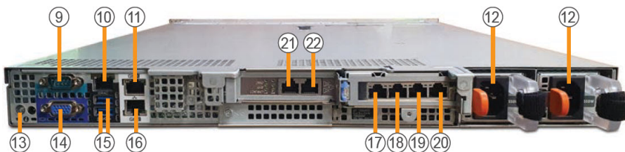
FIGURE 2-6. Deep Discovery Inspector 520E-B/1200E-B Back Panel
