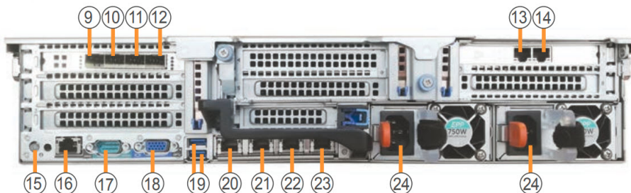
FIGURE 2-7. Deep Discovery Inspector 4200-I/9200-I Back Panel
