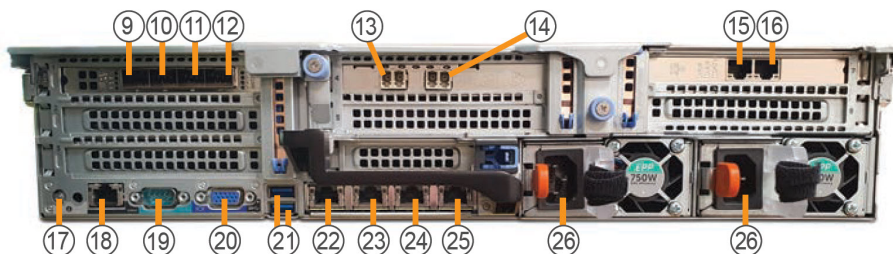
FIGURE 2-9. Deep Discovery Inspector 4200E-I/9200E-I Back Panel
