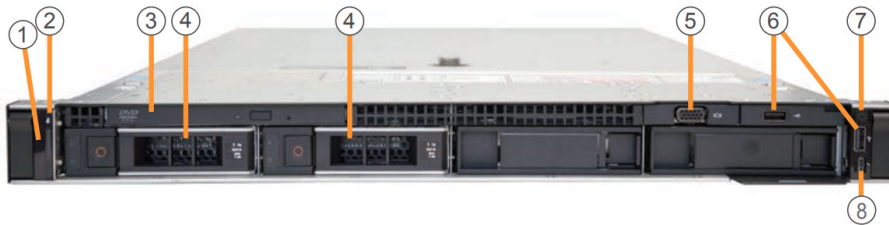
FIGURE 2-2. Deep Discovery Inspector 520/520E/1200/1200E Front Panel
