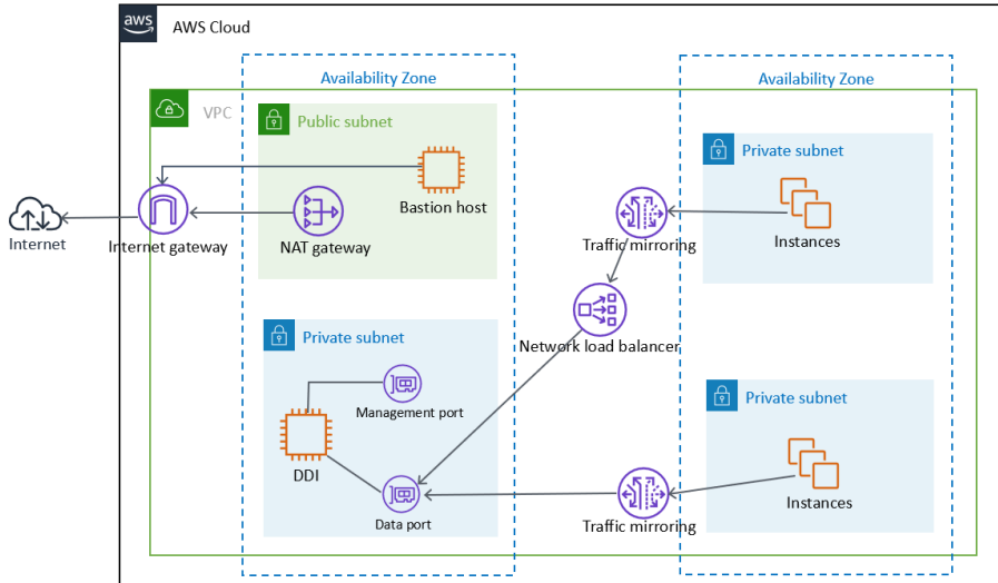
FIGURE 2-1. Deployment Architecture
