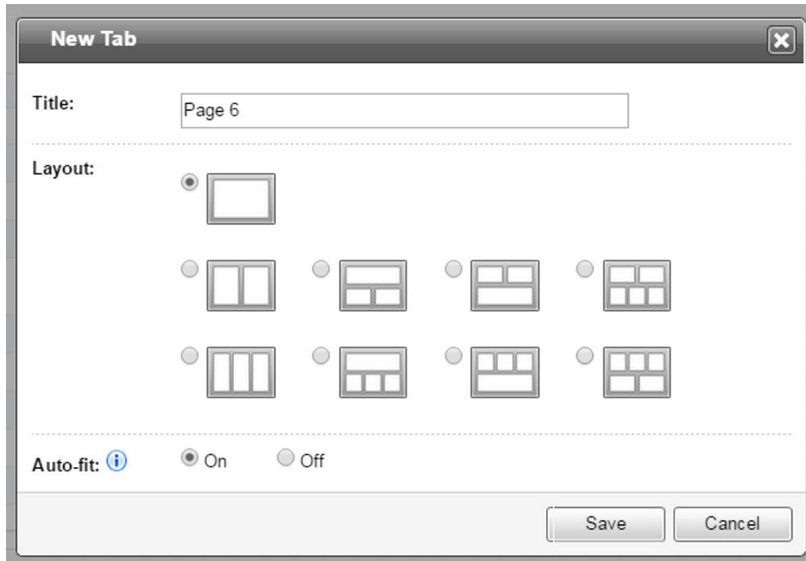
FIGURE 3-2. New Tab
