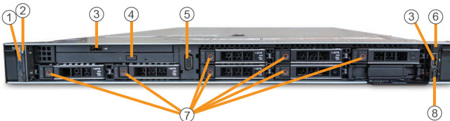
FIGURE 1-2. Front Panel
