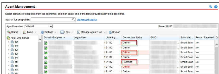
FIGURE 15-2. Agent tree displaying Security Agent connection status with the Apex One server
